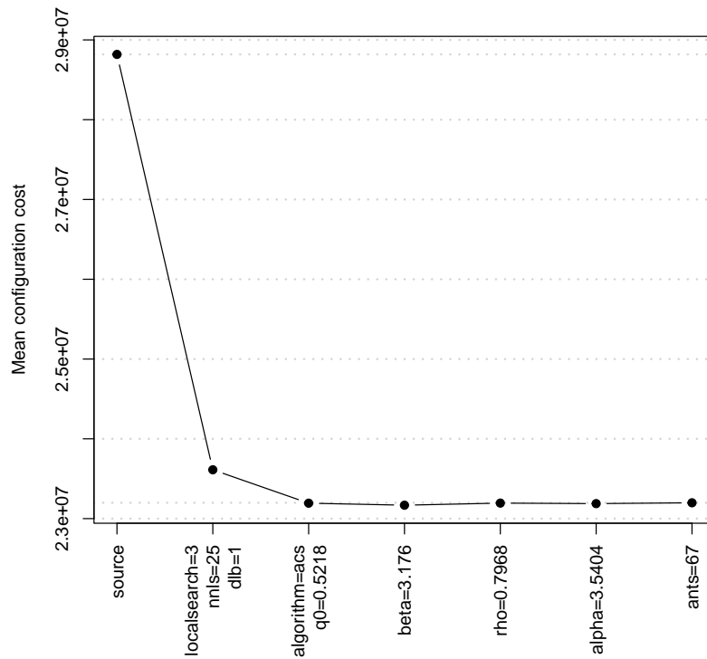
Figure 9: Example of plot generated by plotAblation() .
